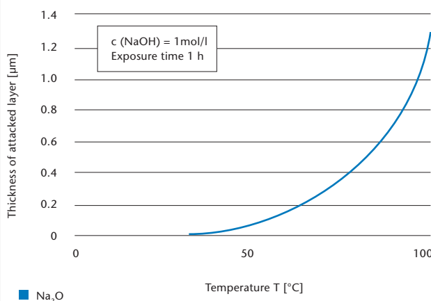
Alkali resistance of BOROFLOAT® 33 as a function of temperature (moderate loss of mass).
